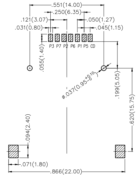
Recommended P.C.Board Layout General tolerances: ±.002(0.05)
