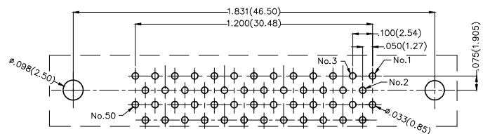
Recommended P.C.Board Layout General Tolerances: ±0.05mm
