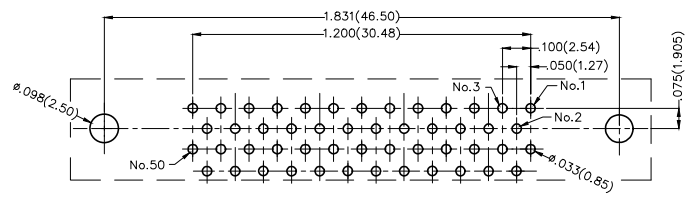
Recommended P.C.Board Layout General Tolerances: ±0.05mm
