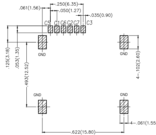
Recommended P.C.Board Layout GENERAL TOLERANCES: ±0.05mm
