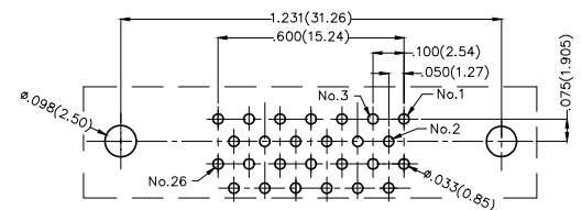
Recommended P.C.Board Layout General Tolerances: ±0.05mm
