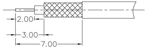
Recommended cable stripping dimensions
