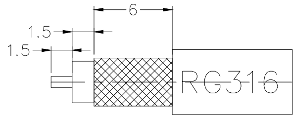
Recommended cable stripping dimension
