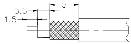
Recommended cable stripping dimension
