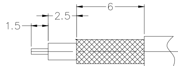
Recommended cable stripping dimension
