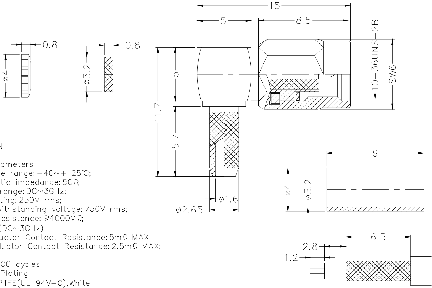
Recommended cable stripping dimension
