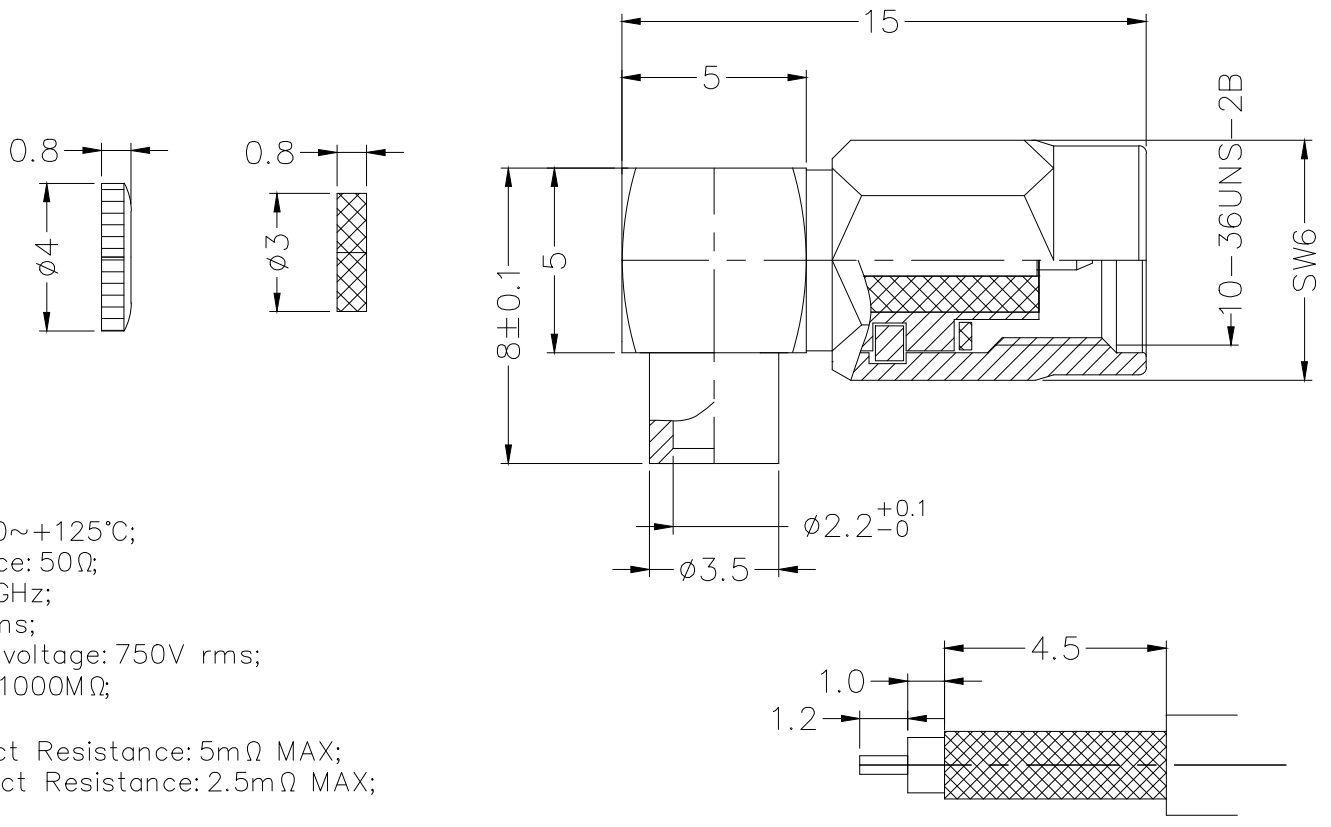
Recommended cable stripping dimension
