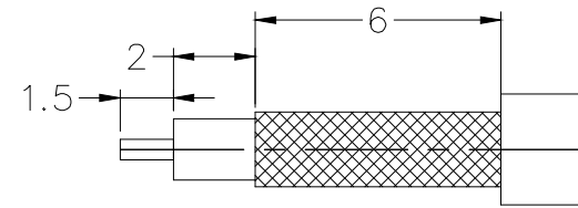
Recommended cable stripping dimension
