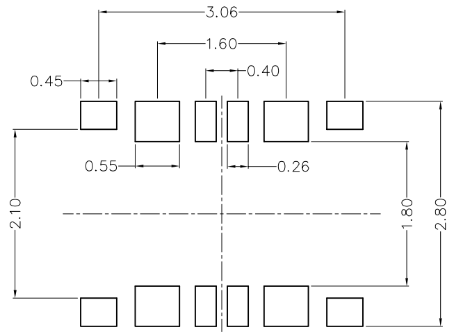
Recommended P.C.Board Layout General tolerances: ±0.05
