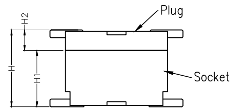
Mating Section
