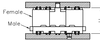
ASSEMBLY
