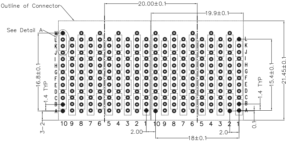
Recommended P.C.Board Layout Tolerances: ±0.05
