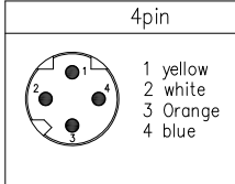
WIRING CHART(MALE Front View)
