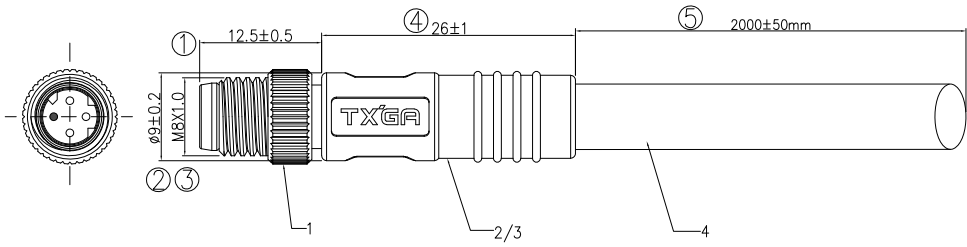
WIRING CHART(MALE Front View)
