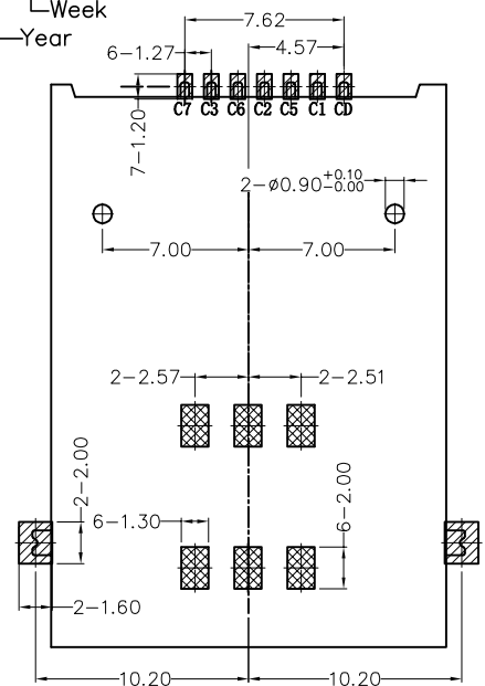
Recommended P.C.Board Layout General Tolerances: ±0.05mm
