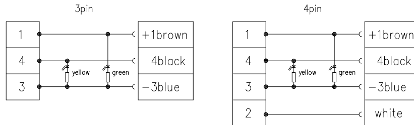
WIRING CHART(FEMALE Front View)
