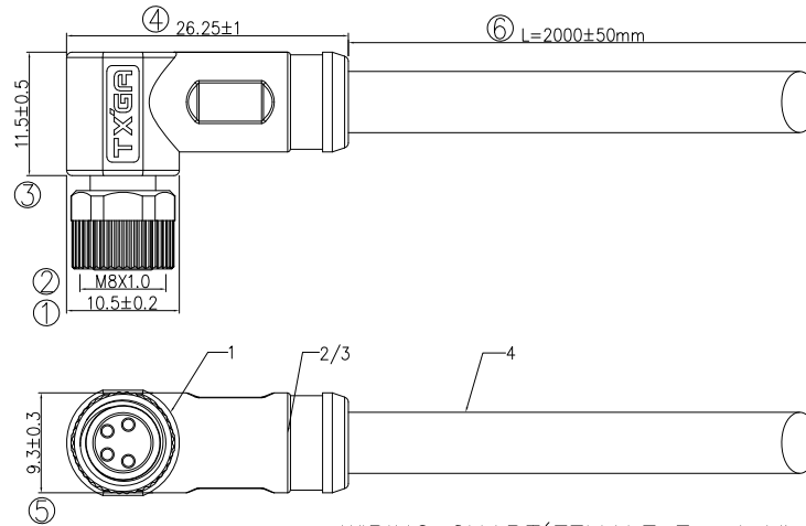
WIRING CHART(FEMALE Front View)
