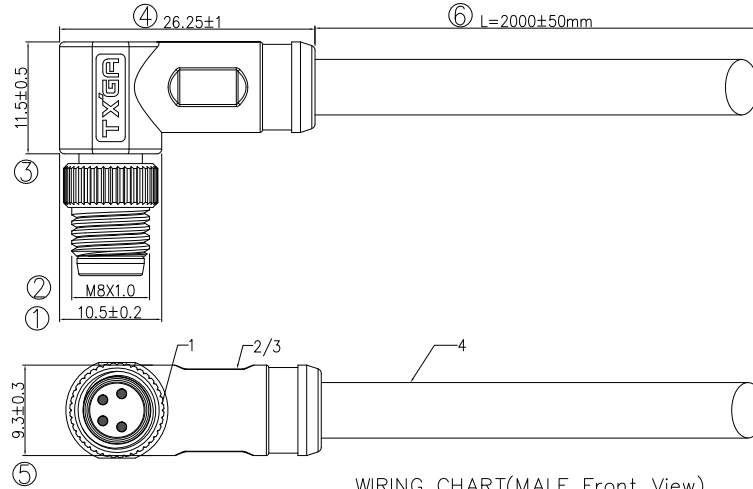
WIRING CHART(MALE Front View)
