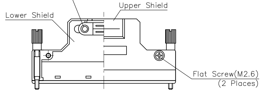
Flat Screw(M2.6) (2 Places)
