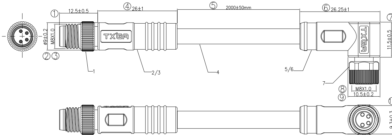
WIRING CHART(MALE Front View)
