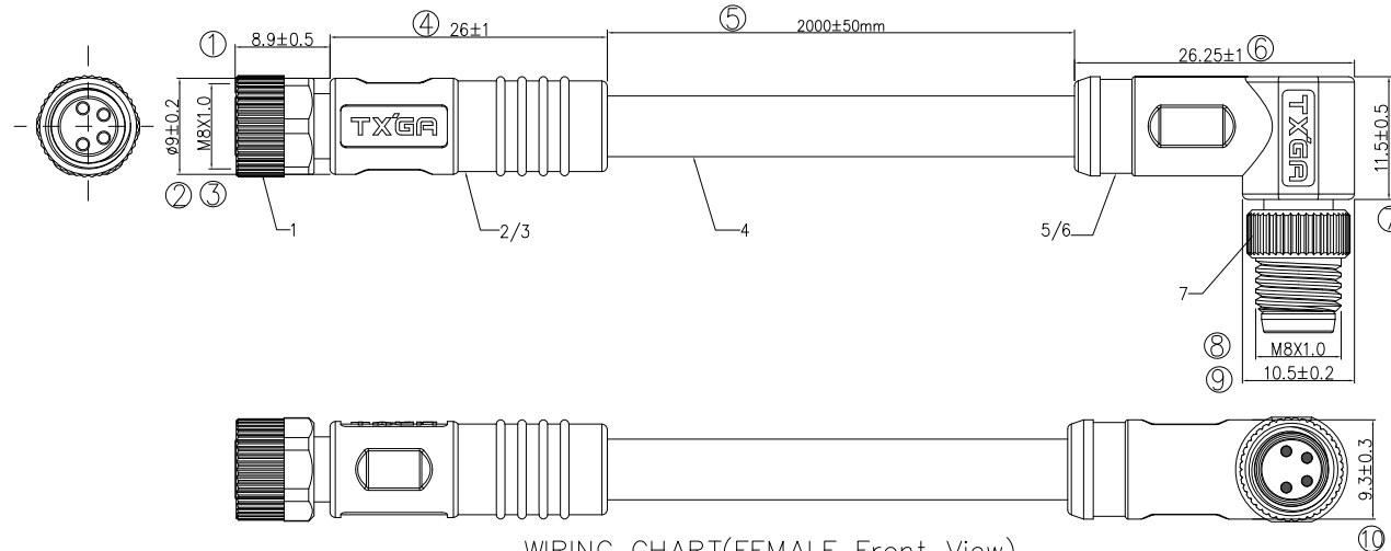
WIRING CHART(FEMALE Front View)
