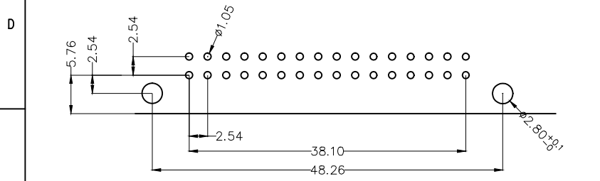
Recommended P.C.Board Layout General Tolerances: ±0.05mm
