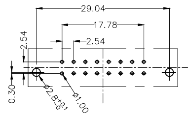
Recommended P.C.Board Layout General Tolerances: ±0.05mm
