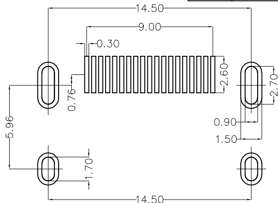
Recommended P.C.Board Layout Tolerance: ±.002(±0.05)
