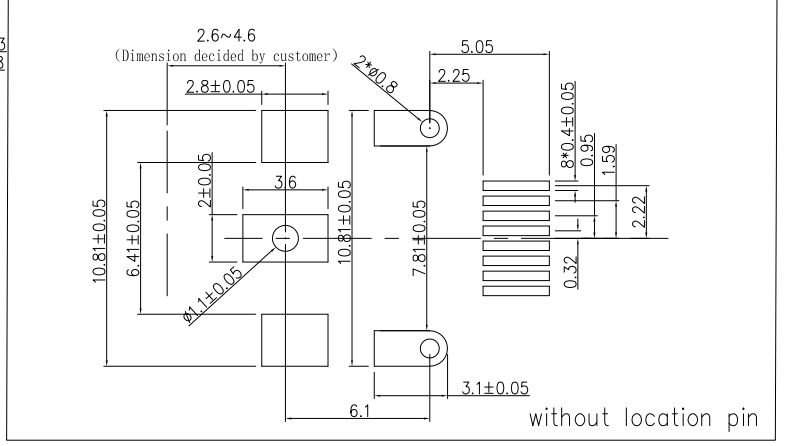
REFERENCE PCB DIMENSIONS
