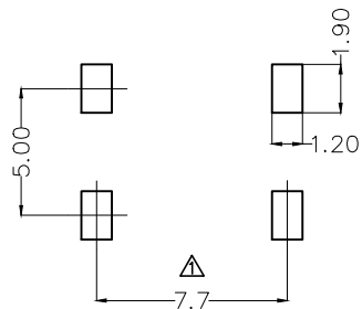
Recommended P.C.Board Layout Tolerance: ±0.05
