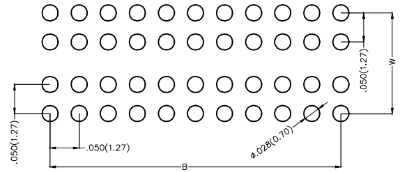
Recommended P.C.Board Layout Tolerances: ±.002(0.05)
