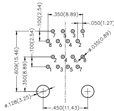
Recommended P.C.Board Layout Tolerances: ±.002(0.05)
