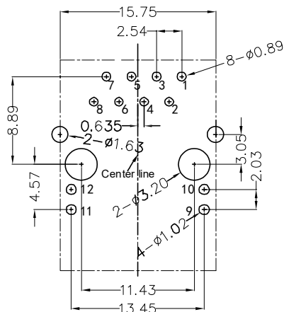
Recommended P.C.Board Layout Tolerances: ±0.05
