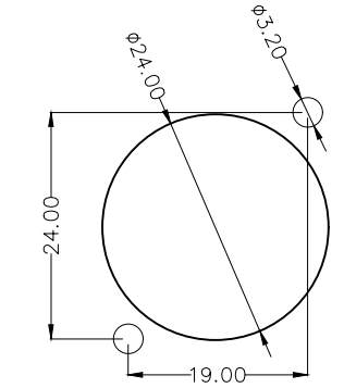
Panel cut out (rear side)
