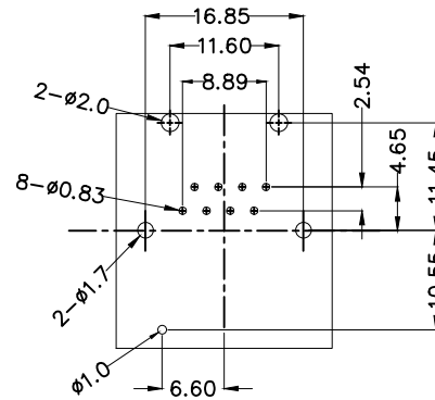
Recommended P.C.Board Layout General tolerances:±0.05
