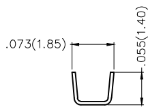
SEC B-B
