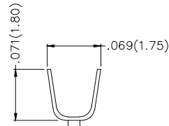
SEC C-C
