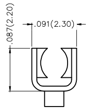
Section C-C
