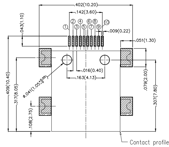
Recommended P.C.Board Layout Tolerances ±.002(0.05)
