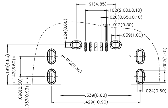
Recommended P.C.Board Layout General Tolerances: ±0.05mm
