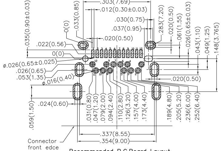
Recommended P.C.Board Layout General Tolerances: ±0.05mm
