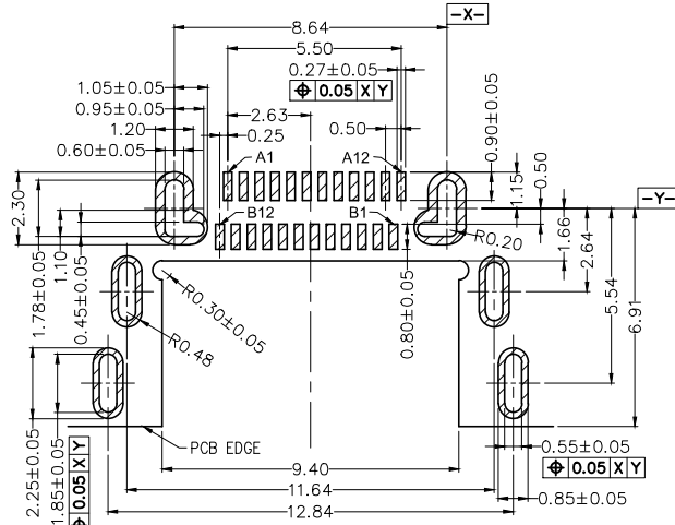
Recommended P.C.Board Layout General Tolerances: ±0.05
