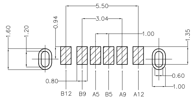
Recommended P.C.Board Layout General tolerances ±0.05mm
