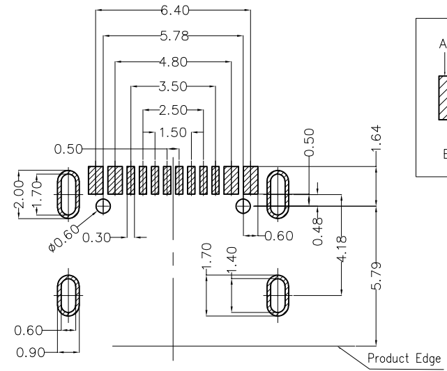
Recommended P.C.Board Layout General tolerances ±0.05mm
