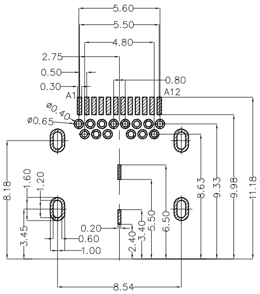
Recommended P.C.Board Layout General tolerances ±0.05mm
